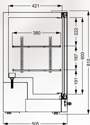
CERVEJEIRA HOME BEER 86 LITROS
