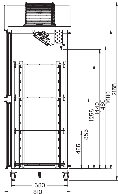
VISA COOLER STORAGE 1900L
