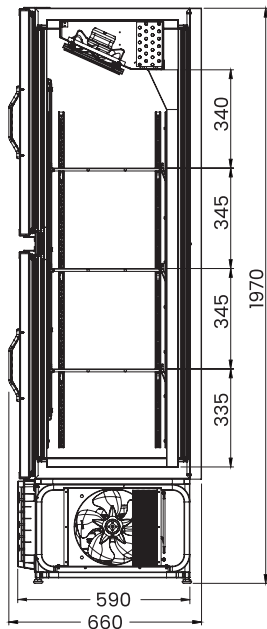
VISA COOLER STORAGE 900L
