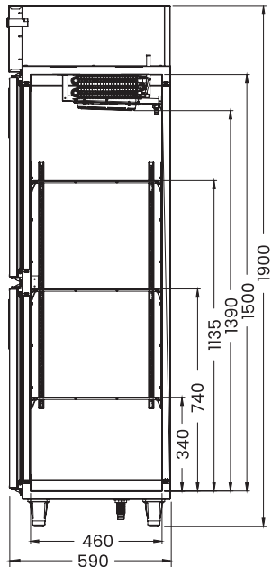
VISA COOLER STORAGE 750L
