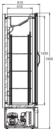
VISA COOLER EXTRA FRIO 300L
