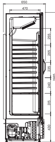
VISA COOLER CARNES 400 VISA COOLER CONGELADOS 400 VISA COOLER SORVETES 400
