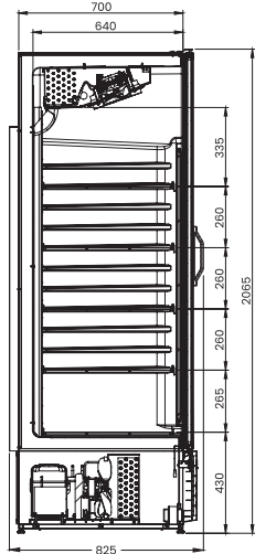
VISA COOLER CONGELADOS 570 VISA COOLER SORVETES 570
