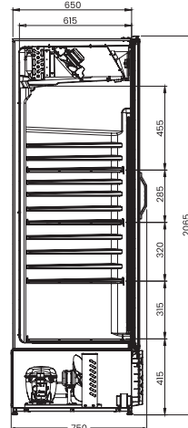
VISA COOLER CERVEJA 570 VISA COOLER CARNE 570
