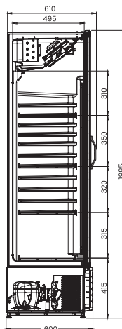
VISA COOLER CERVEJA 400 VISA COOLER MULTIUSO 400
