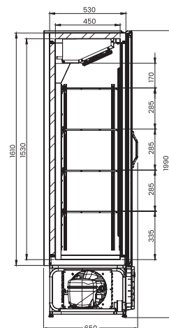
VISA COOLER MULTIPORTAS
