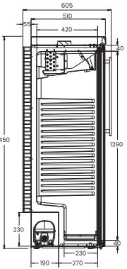
VISA COOLER 230 LITROS
