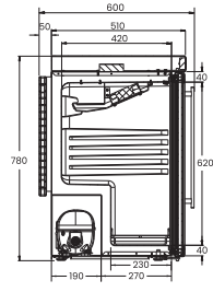
VISA COOLER 86 LITROS
