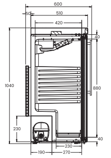
VISA COOLER 130 LITROS
